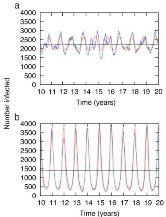
Fig. 1. The effect of seasonal forcing on oscillations in influenza incidence. We simulate disease dynamics in a population of 500,000 people both with (blue) and without (red) demographic stochasticity. \mathcal{R}_0 varies sinusoidally between 9.6 and 10.4. The black curve shows the (nearly invisible) oscillations in incidence that these variations in \mathcal{R}_0 would cause if disease dynamics responded instantaneously to changes in transmission, without resonance or transient fluctuations. (a) Weak resonance. The intrinsic oscillatory period is T \approx 0.59 years (duration of infectiousness 0.02 yr, duration of immunity 4 yr). (b) Strong resonance. T \approx 0.94 yr (duration of infectiousness 0.025 yr, duration of immunity 8 yr). When parameters are drawn at random from the ranges given for \mathcal{R}_0 , D , and L in the text, we find strong oscillations due to resonance (winter peak/summer trough >5 ) for 21% of parameter sets (Fig. 2).
